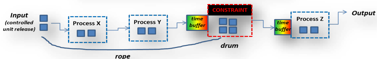
DBR Demonstrated in a Simple Production System
